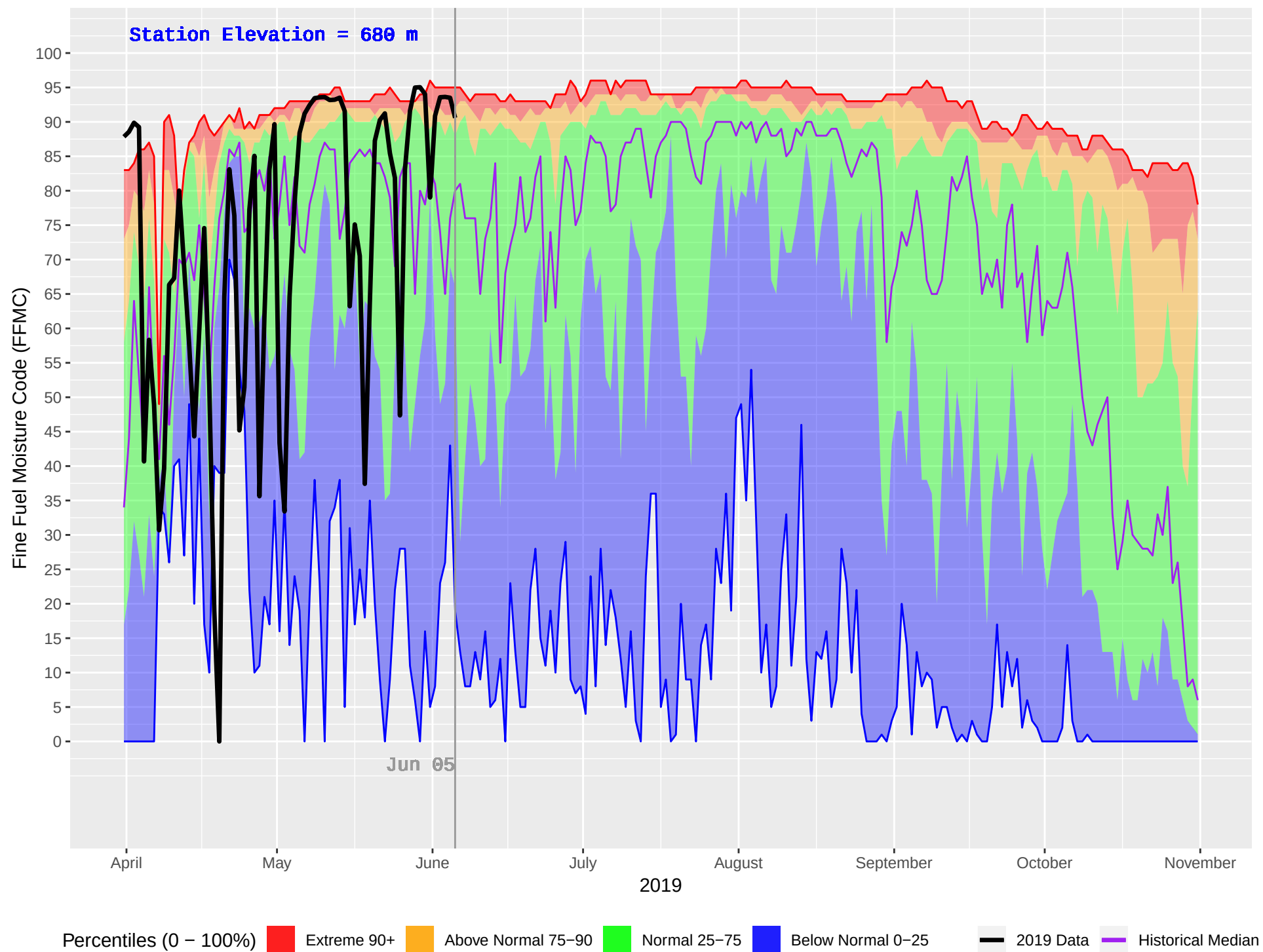
REVELSTOKE (363) : Historical (1995–2018) and Current (2019) Daily Fine Fuel Moisture Code (FFMC)
