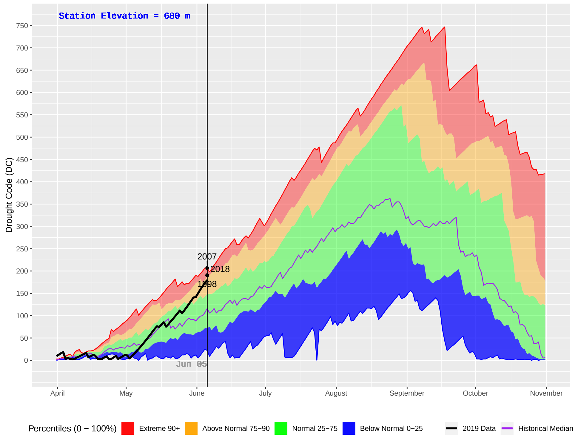
REVELSTOKE (363) : Historical (1995–2018) and Current (2019) Daily Drought Code (DC)
