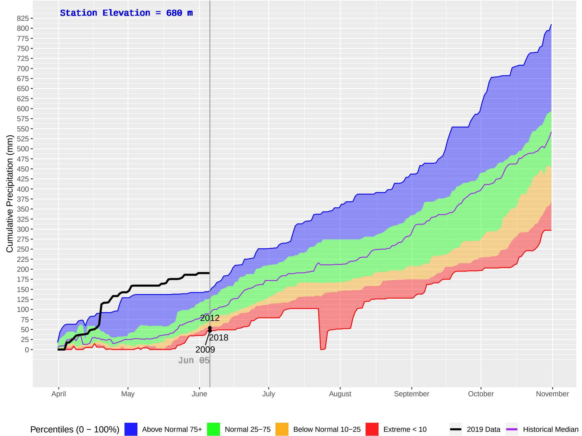
REVELSTOKE (363) : Historical (1995–2018), Current (2019) Daily Cumulative Precipitation
