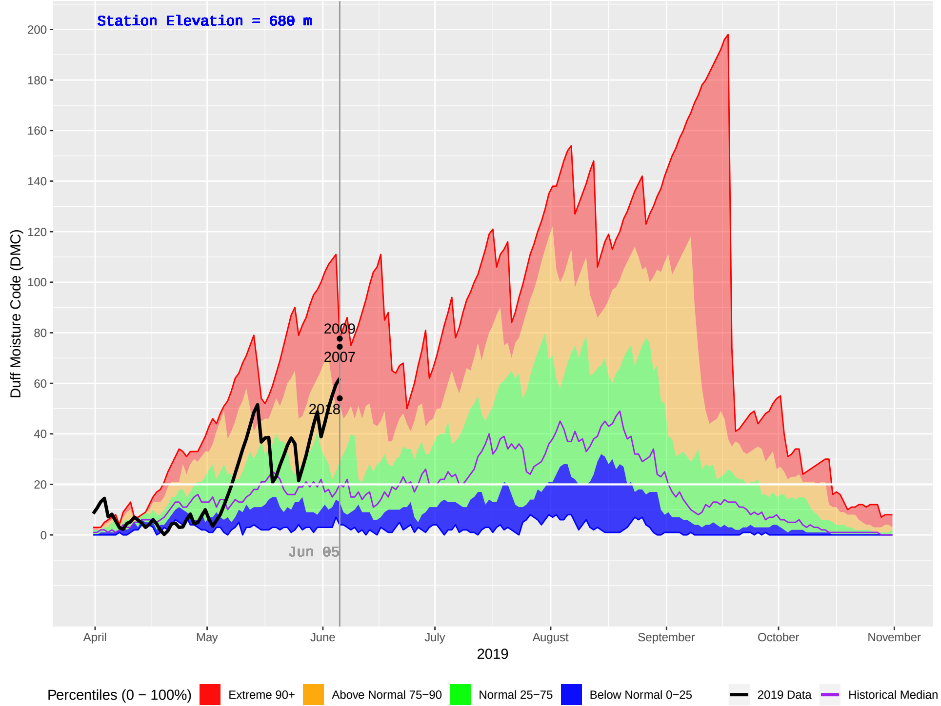
REVELSTOKE (363) : Historical (1995–2018), Current (2019) Daily Duff Moisture Code (DMC)
