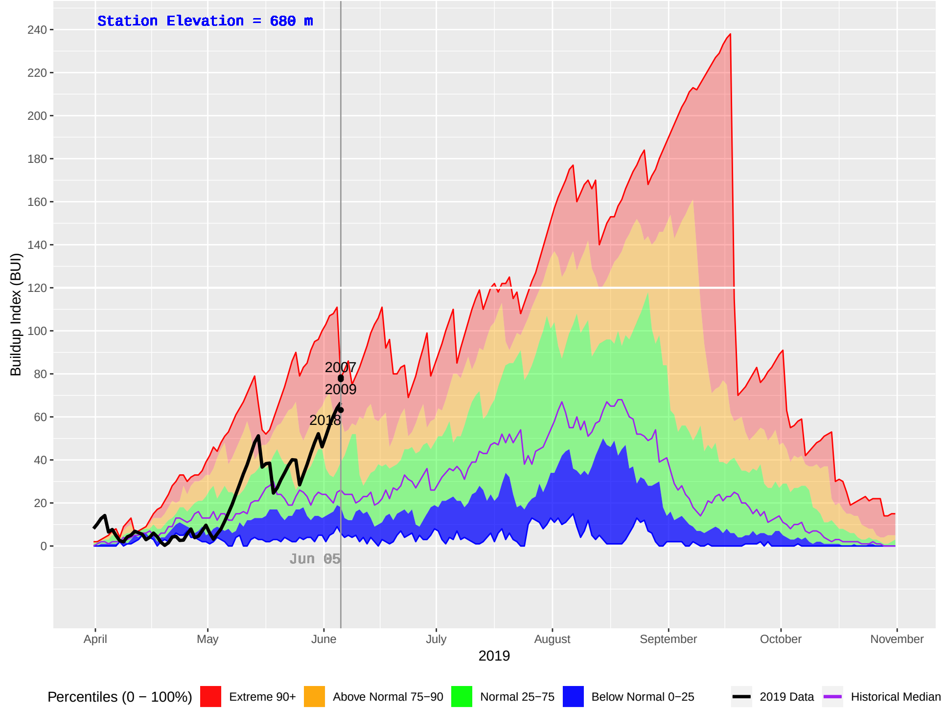
REVELSTOKE (363) : Historical (1995–2018), Current (2019) Daily Buildup Index (BUI)
