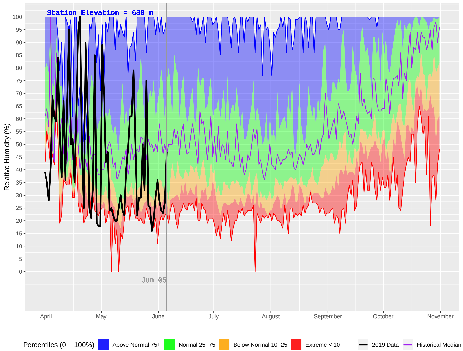
REVELSTOKE (363) : Historical (1995–2018) and Current (2019) Daily Relative Humidity
